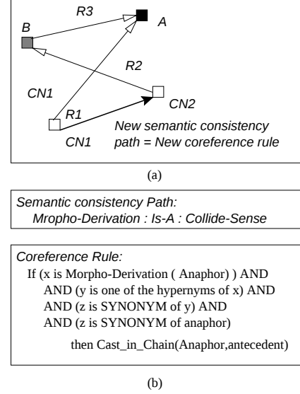
Figure 5: Bootstrapping new rules.
