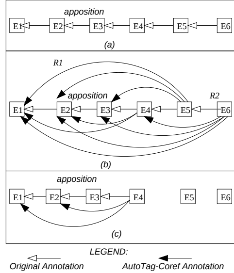
Figure 2: New coreference annotations and the effect of one filter. An example.
